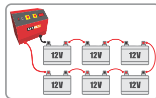
Connected with 6 Batteries (Max)
